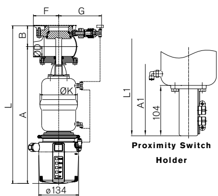
Valve with DELTA CU4
